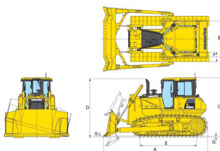
Dimension with SIGMADOZER (D65EX-16) single grouser shoe.
