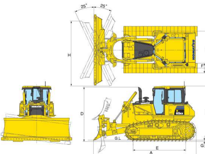
Dimension with Power angle power tilt dozer (D65EX-16) single grouser shoe.
